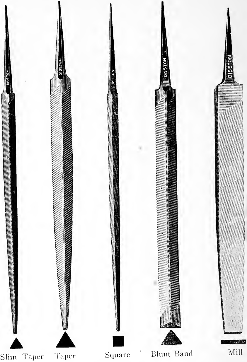
FIG. 96. FILES.
